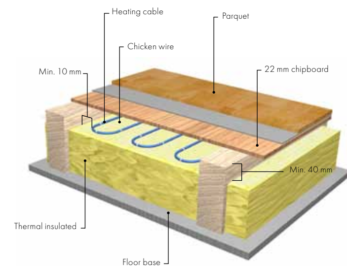
Layer of wooden beams with heating cables
